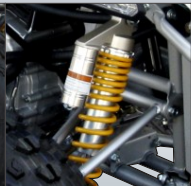
pro gas shocks fitted
